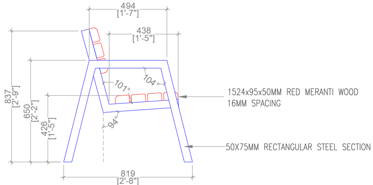
SIDE ELEVATION
